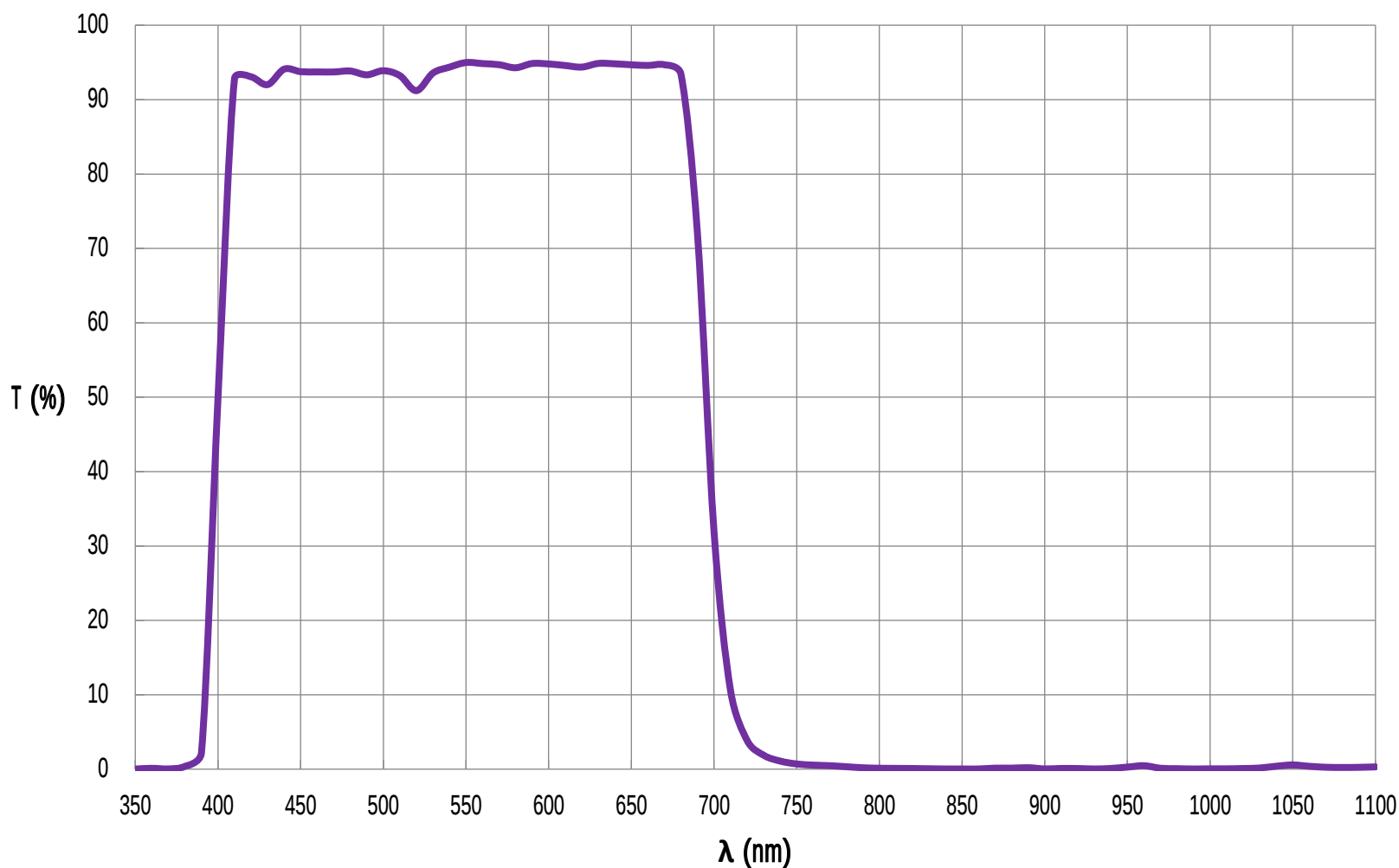
NIR/UV Block-Visible Machine Vision Bandpass Filter, 550nm FOR REFERENCE ONLY
