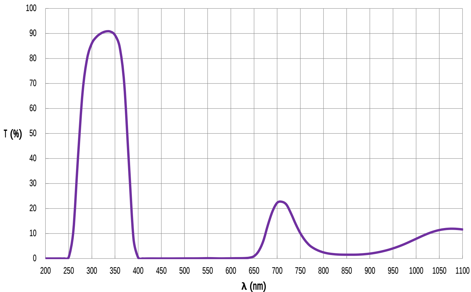
Near-UV Machine Vision Bandpass Filter, 324nm FOR REFERENCE ONLY
