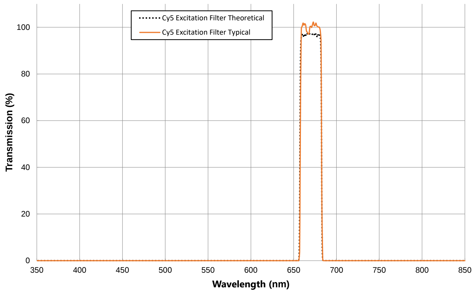
670nm CWL, OD8 High Blocking Bandpass Filter FOR REFERENCE ONLY
