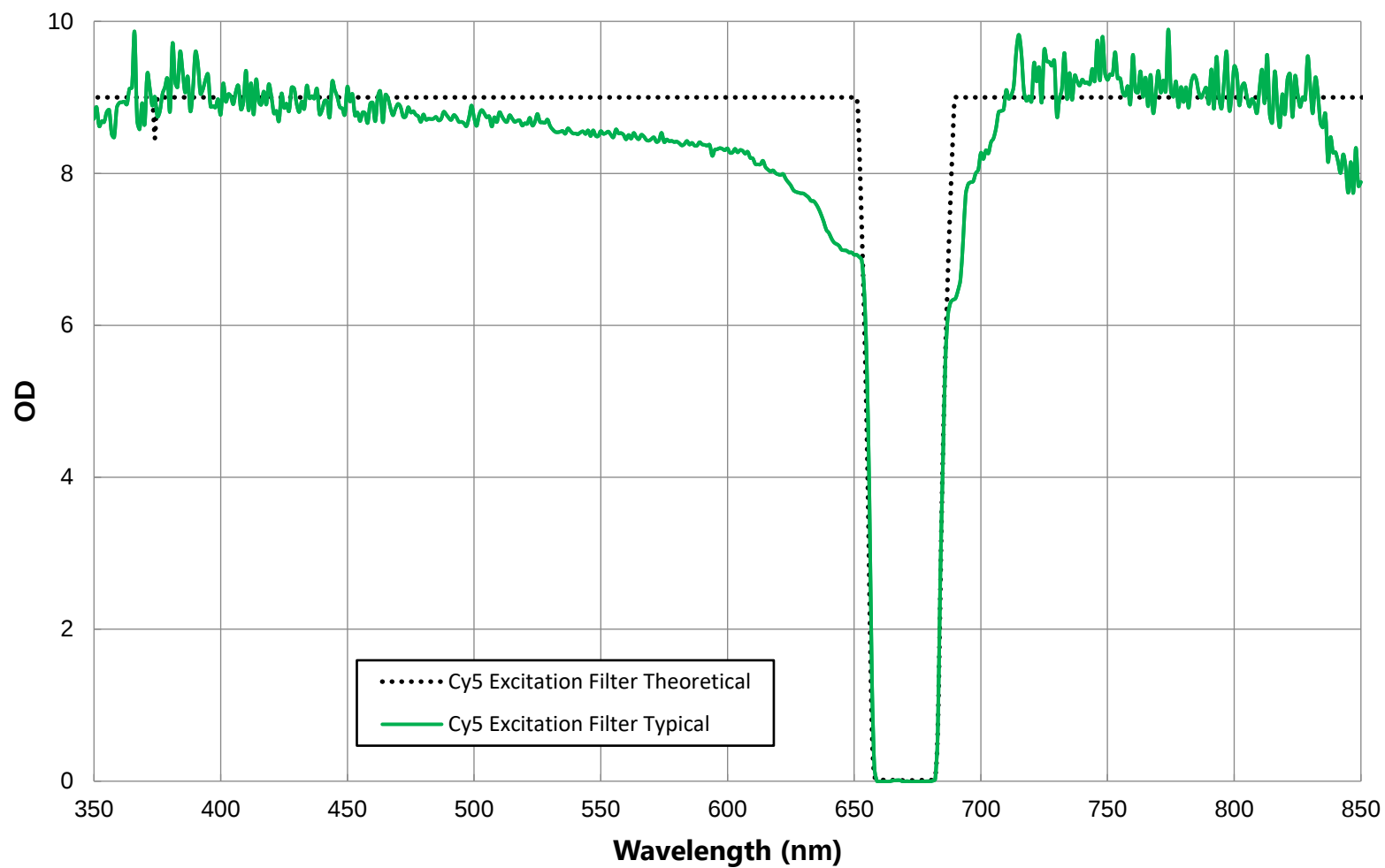
670nm CWL, OD8 High Blocking Bandpass Filter FOR REFERENCE ONLY
