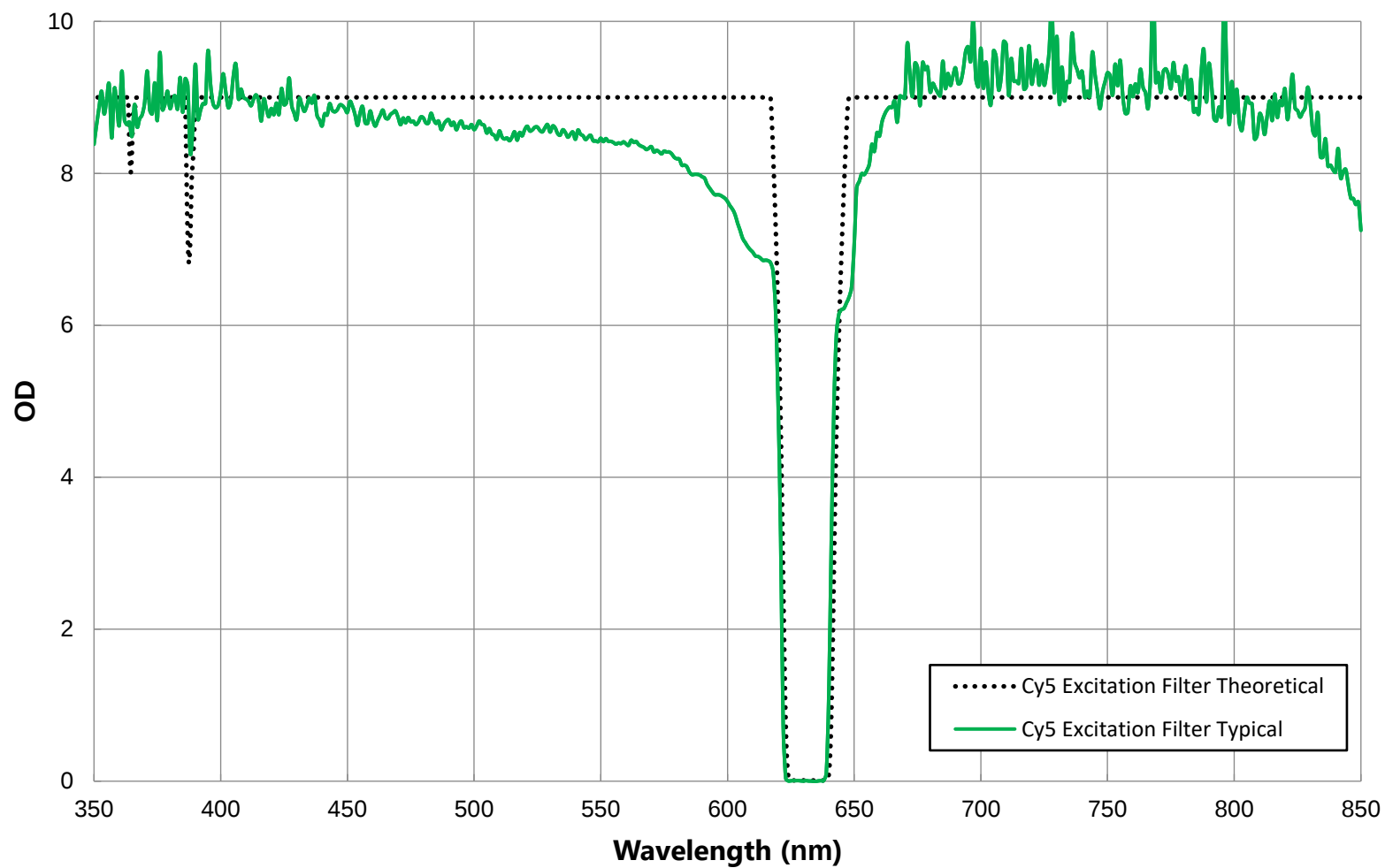
630nm CWL, OD8 High Blocking Bandpass Filter FOR REFERENCE ONLY
