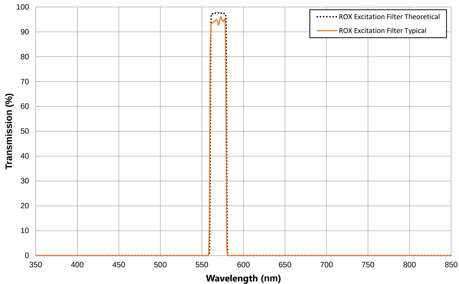
570nm CWL, OD8 High Blocking Bandpass Filter FOR REFERENCE ONLY
