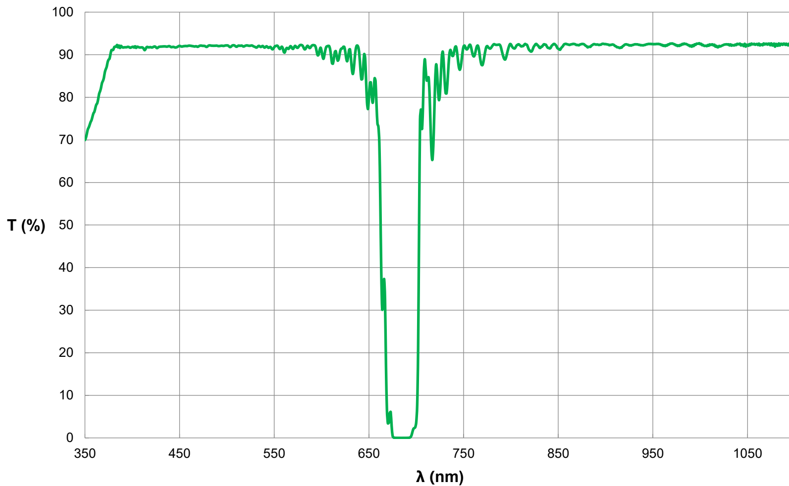
Everix Ultra-Thin OD 4 Notch Filter, 685nm, 12.5mm Diameter FOR REFERENCE ONLY
