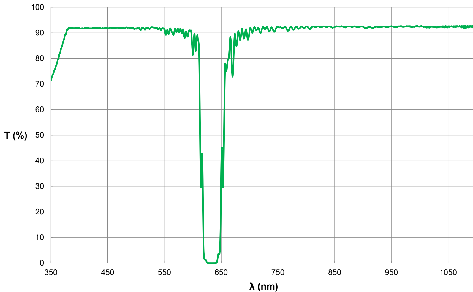
Everix Ultra-Thin OD 4 Notch Filter, 633nm, 12.5mm Diameter FOR REFERENCE ONLY
