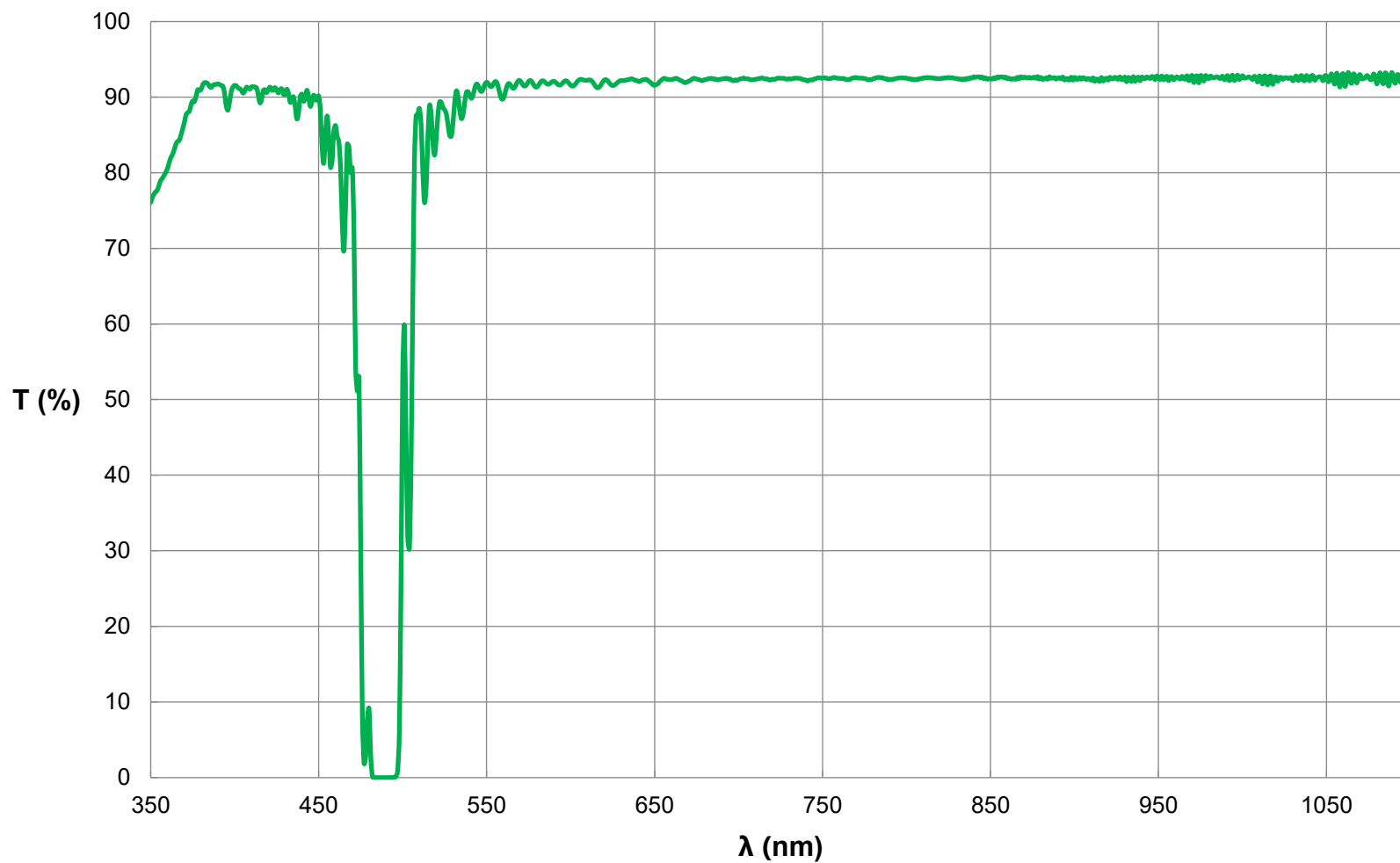
Everix Ultra-Thin OD 4 Notch Filter, 488nm, 12.5mm Diameter FOR REFERENCE ONLY
