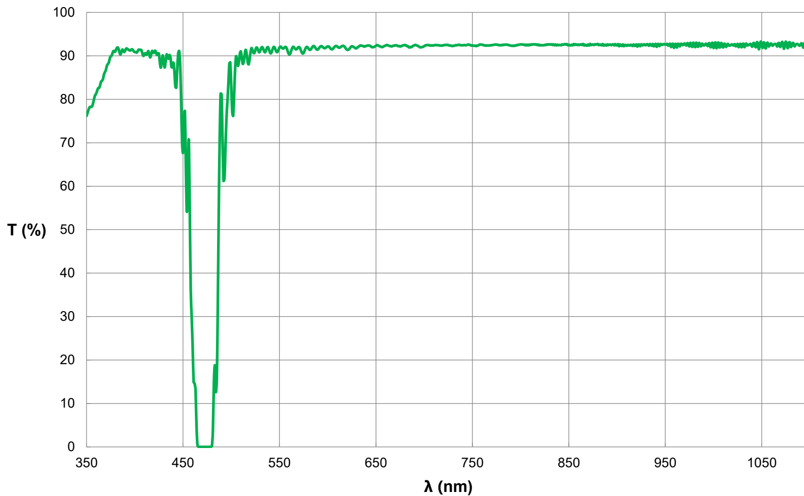
Everix Ultra-Thin OD 4 Notch Filter, 473nm, 12.5mm Diameter FOR REFERENCE ONLY
