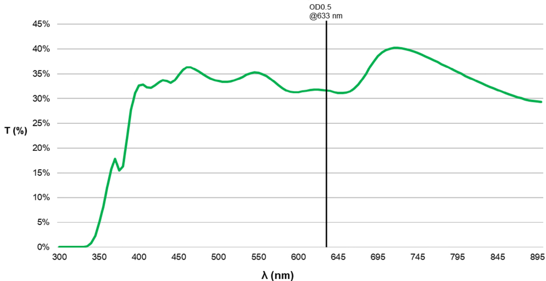
SCHOTT NG5 633 nm 50 Sq., 0.5 OD ND Filter REFERENCE Only
