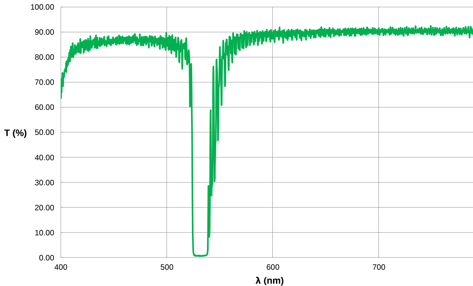
532nm 70x35mm META ® holoOPTIX ® FLEX Notch Filter FOR REFERENCE ONLY
