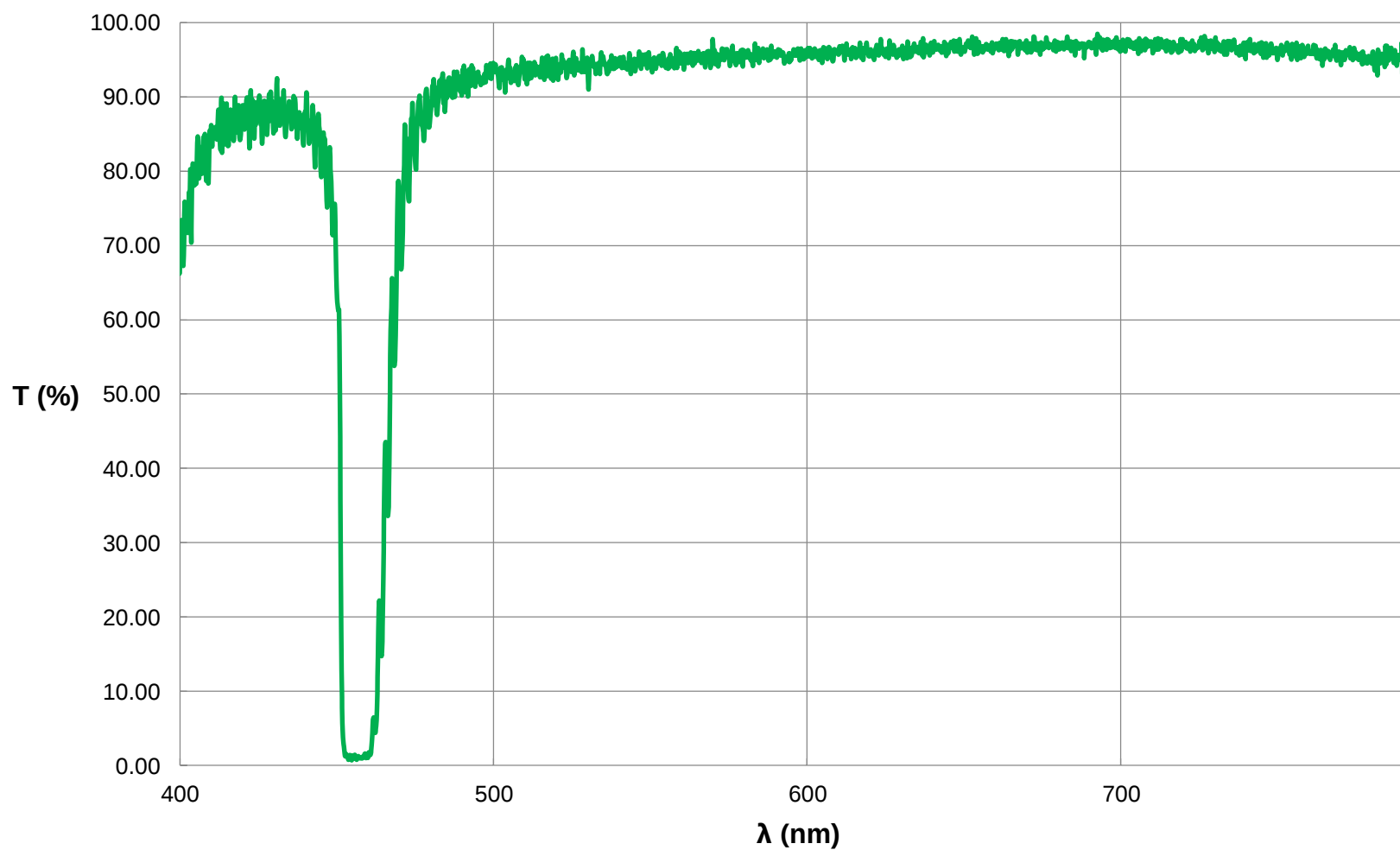
457nm META ® holoOPTIX ® STRATA Notch Filter FOR REFERENCE ONLY
