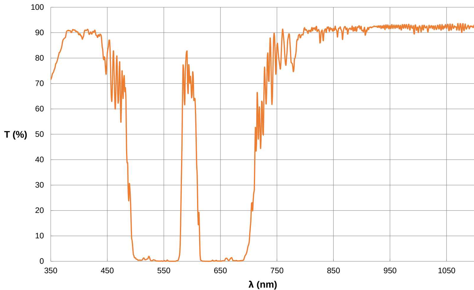
Everix Ultra-Thin Bandpass Filter, 595nm, OD 2.0 FOR REFERENCE ONLY
