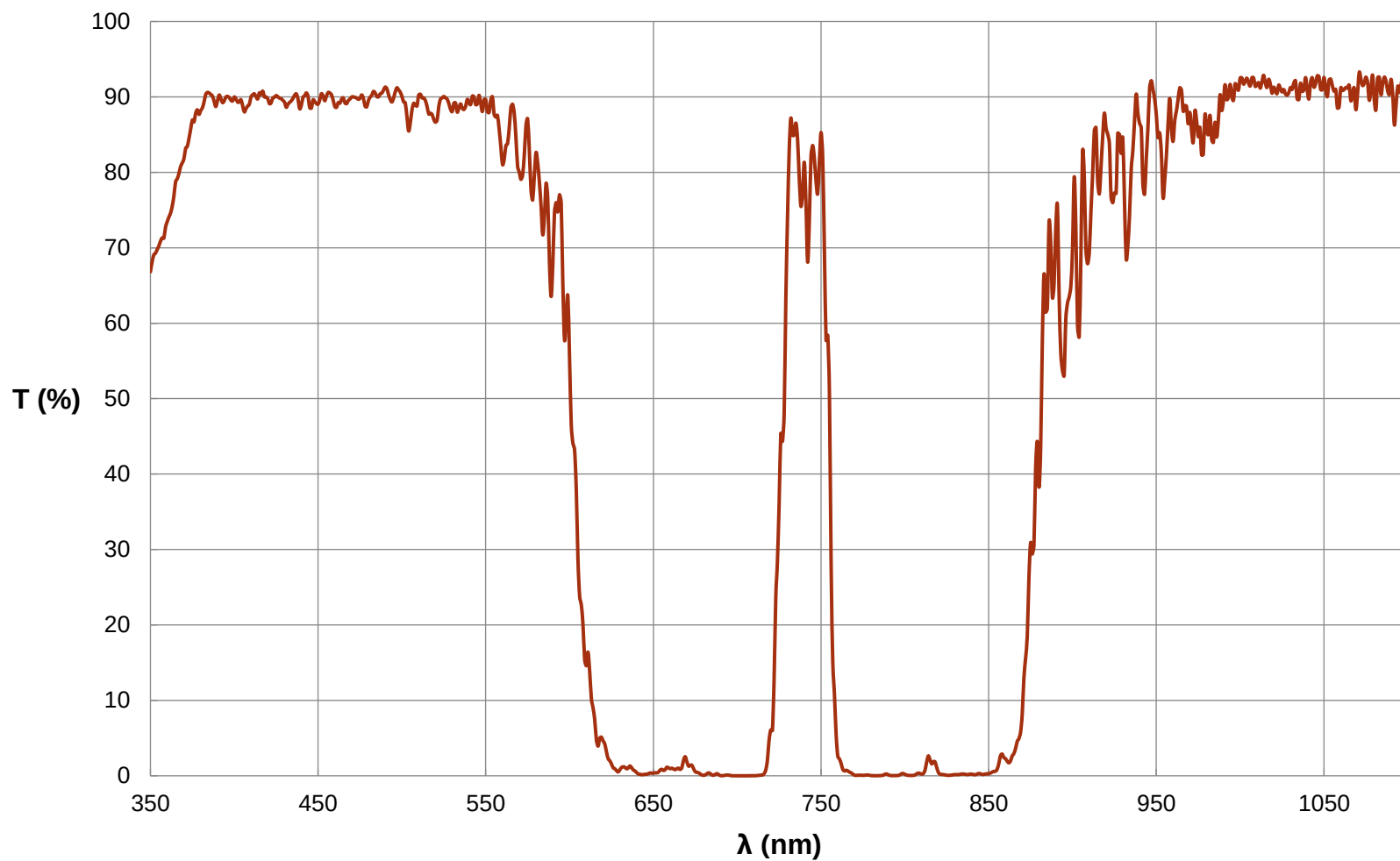
Everix Ultra-Thin Bandpass Filter, 740nm, OD 2.0 FOR REFERENCE ONLY
