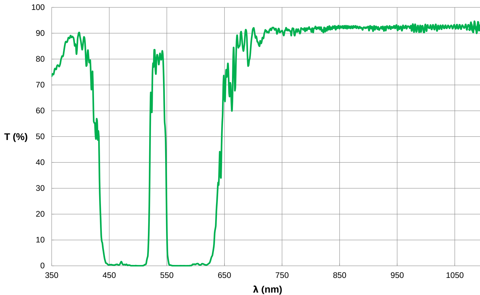
Everix Ultra-Thin Bandpass Filter, 535nm, OD 2.0 FOR REFERENCE ONLY
