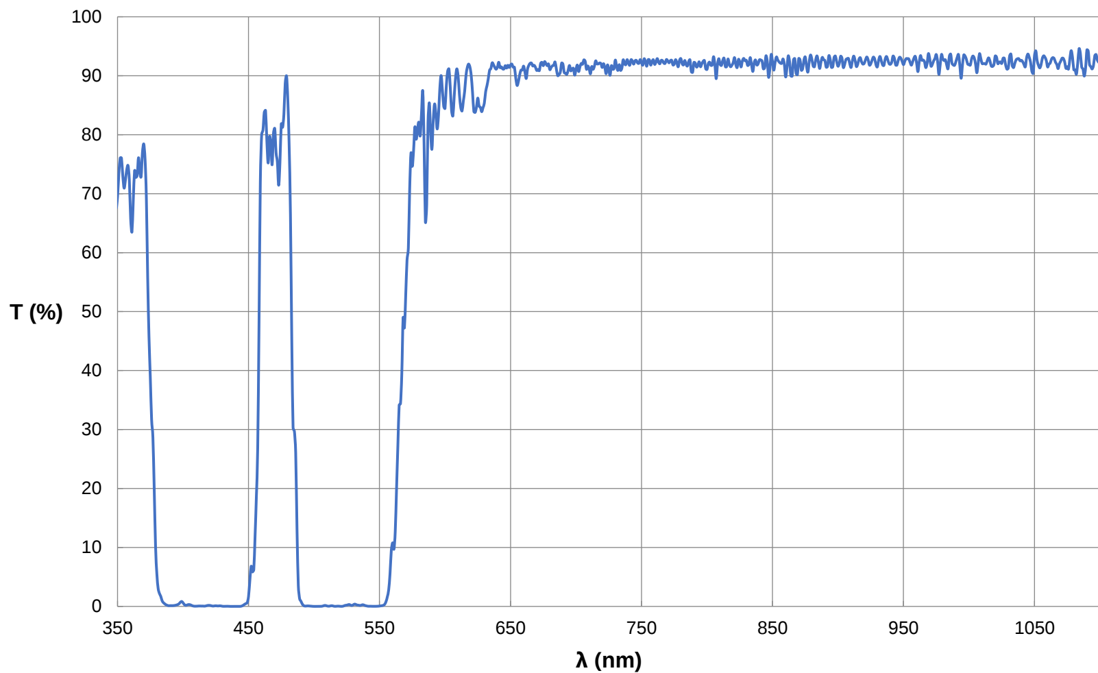
Everix Ultra-Thin Bandpass Filter, 470nm, OD 2.0 FOR REFERENCE ONLY
