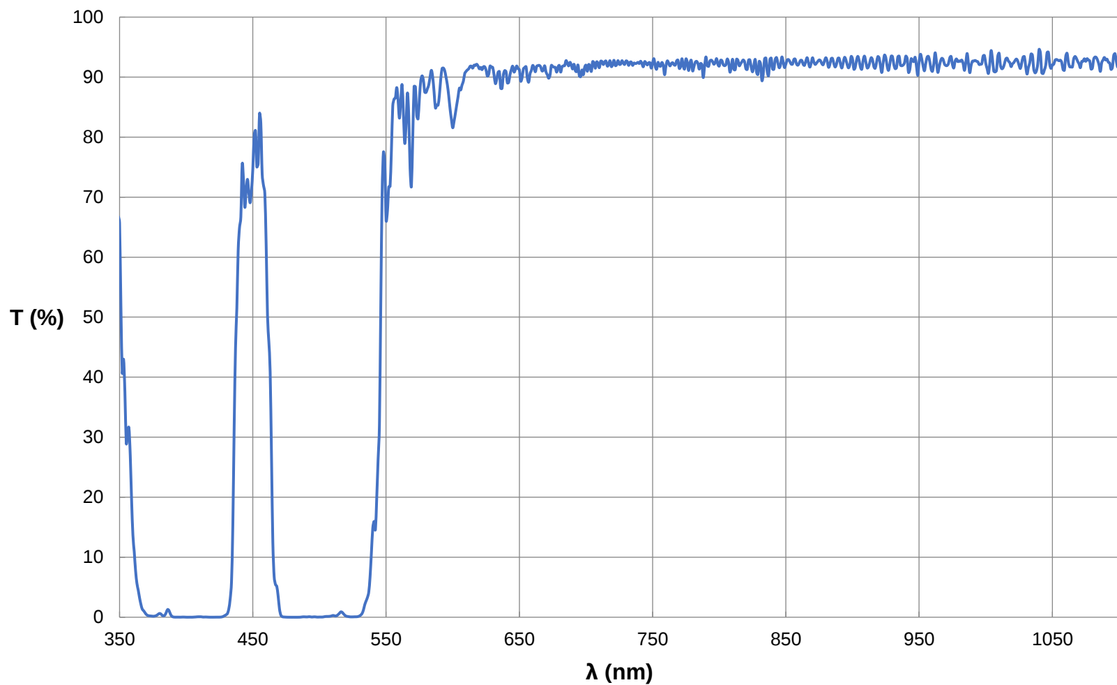
Everix Ultra-Thin Bandpass Filter, 450nm, OD 2.0 FOR REFERENCE ONLY
