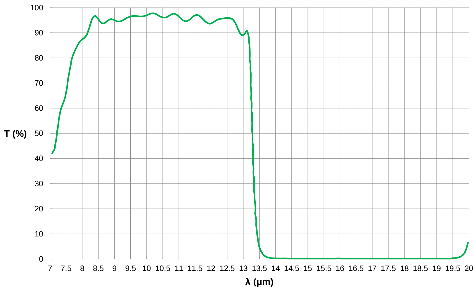
13.3 \mu m Shortpass Filter: OD \geq 3.0 Coating Performance FOR REFERENCE ONLY
