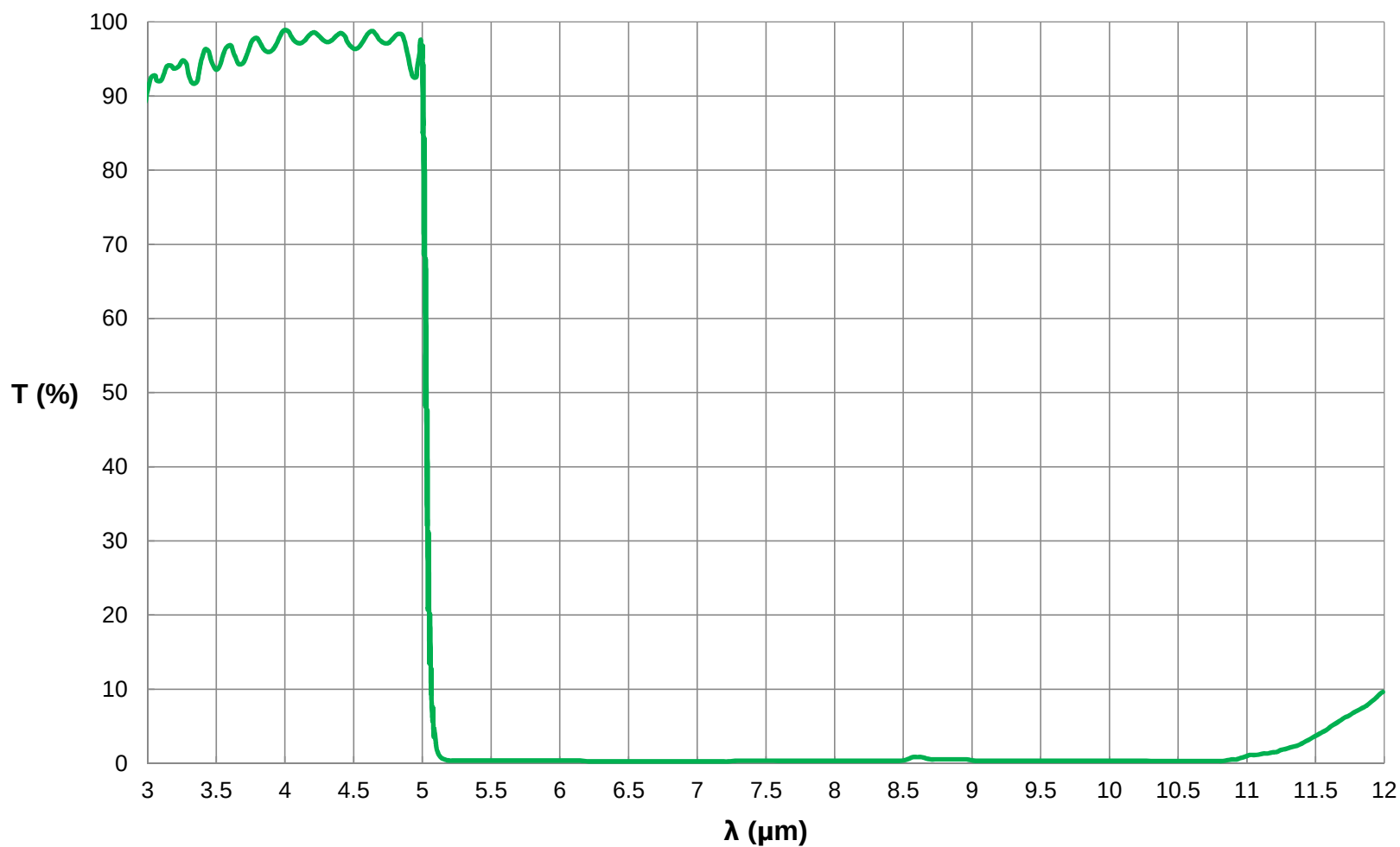
5.0 \mu m Shortpass Filter: OD \geq 3.0 Coating Performance FOR REFERENCE ONLY
