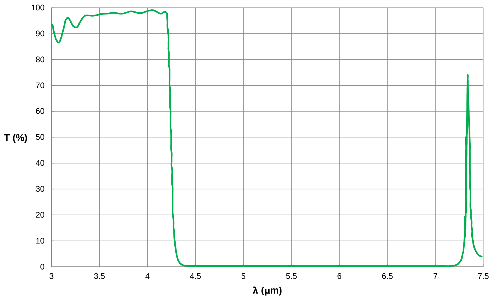
4.25 \mu m Shortpass Filter: OD \geq 3.0 Coating Performance FOR REFERENCE ONLY
