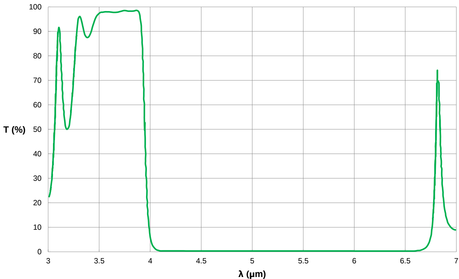
3.95 \mu m Shortpass Filter: OD \geq 3.0 Coating Performance FOR REFERENCE ONLY
