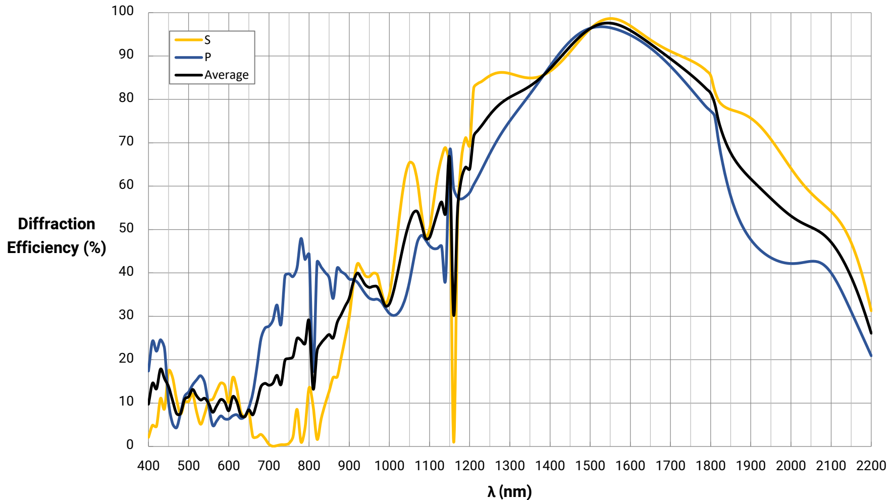
Diffraction Efficiency Curve
